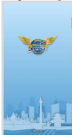
Gambar 11 Tampilan E-Signal
